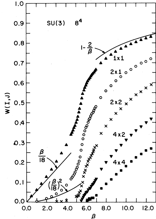
FIG. 1. The Wilson loops W(I, J) for pure SU(3) gauge theory on an 8^4 lattice as a function of the inverse coupling constant squared \beta . The solid upward triangles represent I = J = 1 , the open circles represent I = 2, J = 1 , the crosses represent I = J = 2 , the solid downward triangles represent I = 4, J = 2 and the solid squares represent I = J = 4 . The curves represent the leading-order strong- and weak-coupling expansions of Eqs. (1) and (2), respectively.
