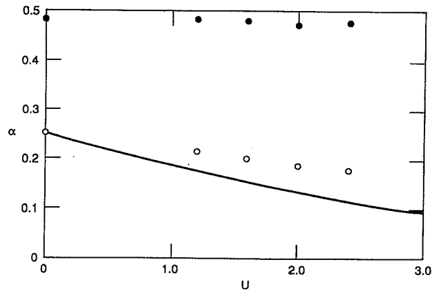
FIG. 1. The behavior of the densities \langle n_{i\uparrow} \rangle (solid points) and \langle n_{i\uparrow} n_{i\downarrow} \rangle (open points) as a function of the coupling U . The other parameters are \beta=1 , K=1 , and h=\mu=0 . The solid curve represents the exact solution for vanishing K . The statistical errors are approximately the size of the points. The fact that \langle n_{i\uparrow} \rangle is less than 0.5 is a consequence of N_t being finite.
