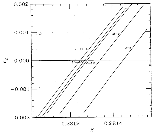
FIG. 1. The ratio r_E defined in Eq. (6) in the vicinity of the Ising critical point. The series expansion for this quantity was Padé approximated in z = 3u^2/(1+3u^2) as the ratio of two polynomials, and the curves are labeled by the highest power of z appearing in the numerator.
