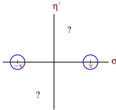
Figure 3: The circles in this figure enclose the two minima in the \sigma, \eta' plane located at \sigma = \pm v and \eta' = 0 . Can we find any other minima?
