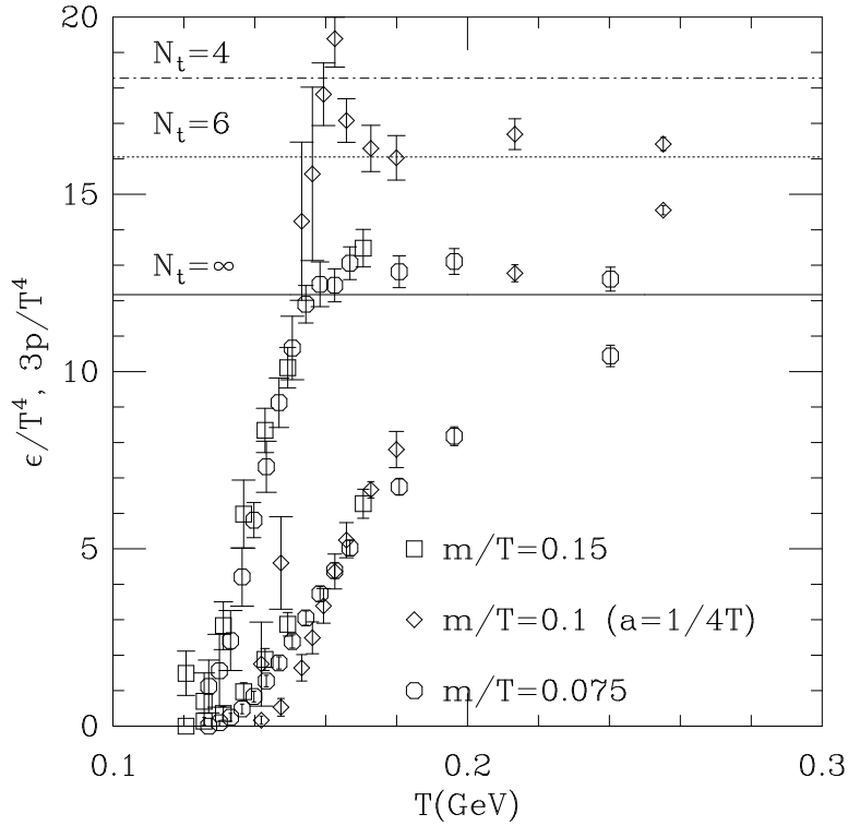
FIGURE 3. The energy and pressure of the æther show a dramatic structure at a temperature of about 170–190 MeV. The lattice is a unique theoretical tool for the study of this transition to a quark-gluon plasma (From Ref. [14]).
