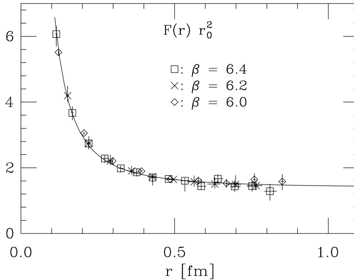
FIGURE 2. The force between two quarks does not fall to zero as the distance increases. This is the confinement phenomenon. (From Ref. [12]).
